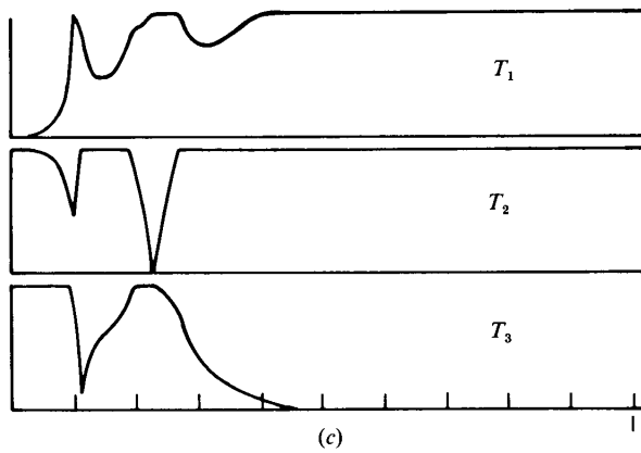
FIGURE 3 ( a, b, c ). For caption see facing page.
