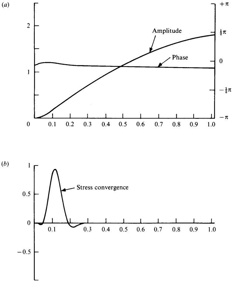
FIGURE 5. (a) Amplitude and phase of incident plus reflected wave (i.e. total wave field) vs. z . (b) Convergence of Reynolds stress vs. z . ( k = 1 ; c_r = 0.1 ; Re = 10000 .)
