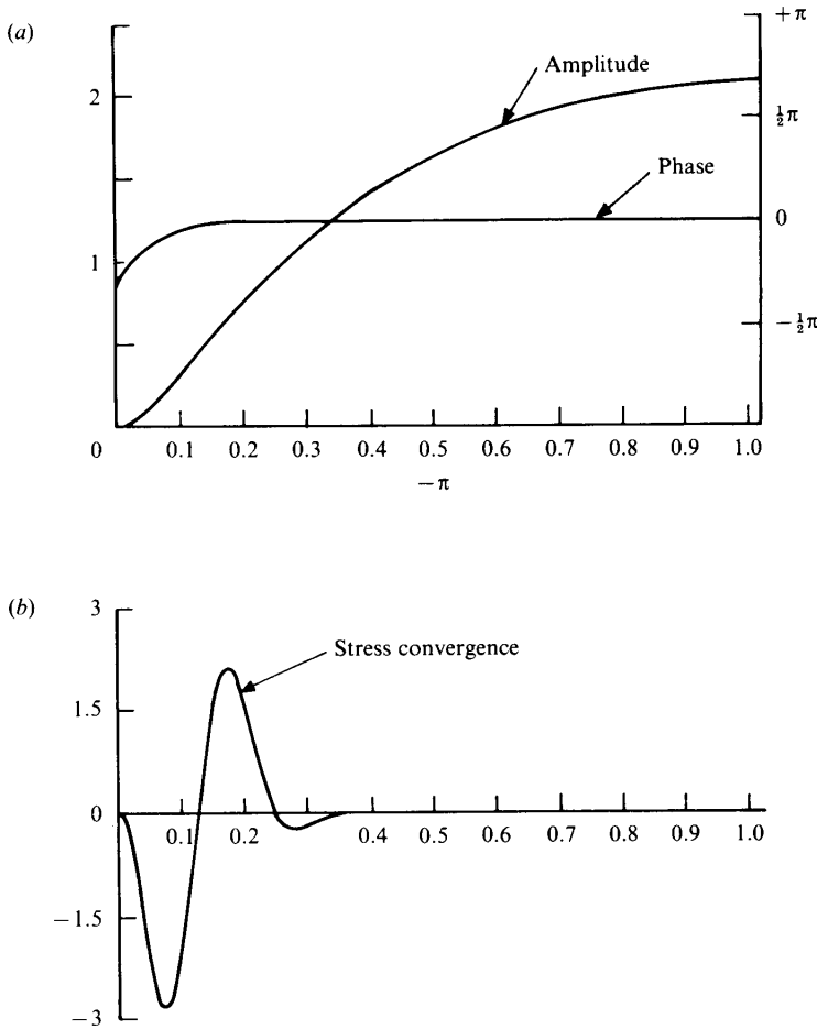
FIGURE 9. Same as figure 5 but for k = 1.093 and c_r = 0.2463 .
