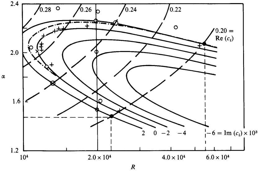
FIGURE 1. Curves of constant amplification, \text{Im}(c) = \text{constant} (solid line). Curves of constant phase velocity, \text{Real}(c) = \text{constant} (dashed line). From Grosch & Salwen 1968.
