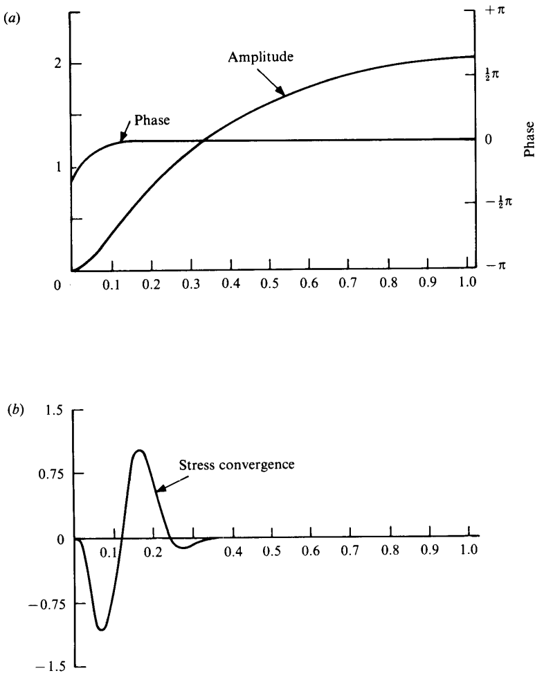
FIGURE 6. Same as figure 5 but for k = 1 and c_r = 0.2375 .
