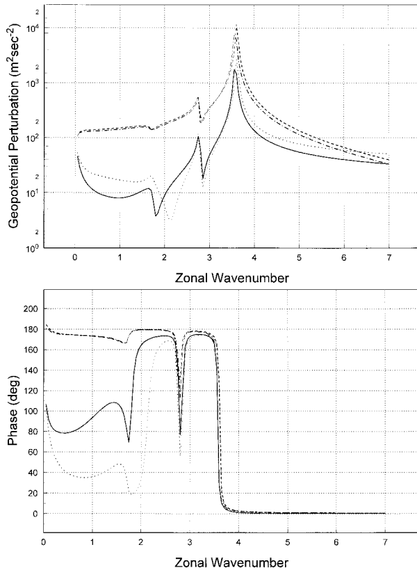
FIG. 1. Response to 100-m surface forcing as a function of zonal wavenumber s . (a) Amplitude of response; (b) phase of response. — corresponds to surface for unadjusted basic state, ... corresponds to surface for adjusted basic state, -- corresponds to 10 km for unadjusted basic state, and - corresponds to 10 km for adjusted basic state. The illustrated results correspond to high resolution and low damping.
