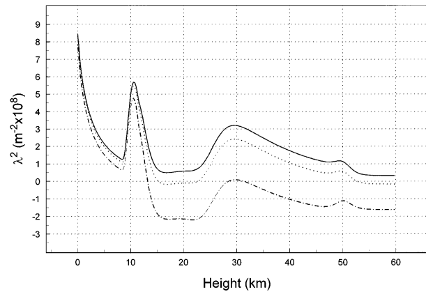
FIG. 4. Approximate index of refraction as a function of height. — corresponds to s = 1 ; ·· corresponds to s = 2 ; and -- corresponds to s = 3.6 . The illustrated results are for unadjusted basic state.
