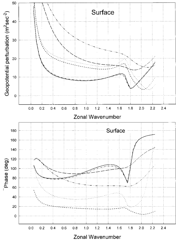
FIG. 2. Surface response to 100-m surface forcing as a function of zonal wavenumber s . (a) Amplitude; (b) phase. — corresponds to high resolution, low damping, and unadjusted basic state; ... corresponds to high resolution, low damping, and adjusted basic state; -- corresponds to low resolution, low damping, and unadjusted basic state; - corresponds to low resolution, low damping, and adjusted basic state; — corresponds to high resolution, high damping, and unadjusted basic state; and --- corresponds to high resolution, high damping, and adjusted basic state.
