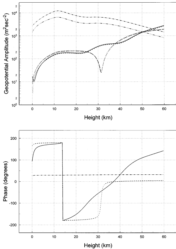
FIG. 3. Vertical structure of response for s = 1 , s = 2 , and s = 3.6 . (a) Amplitude; (b) phase. — corresponds to s = 1 for adjusted basic state; - corresponds to s = 2 for adjusted basic state; -- corresponds to s = 3.6 for adjusted basic state; - corresponds to s = 1 for unadjusted basic state; — corresponds to s = 2 for unadjusted basic state; and --- corresponds to s = 3.6 for unadjusted basic state. The illustrated results correspond to high resolution and low damping.
